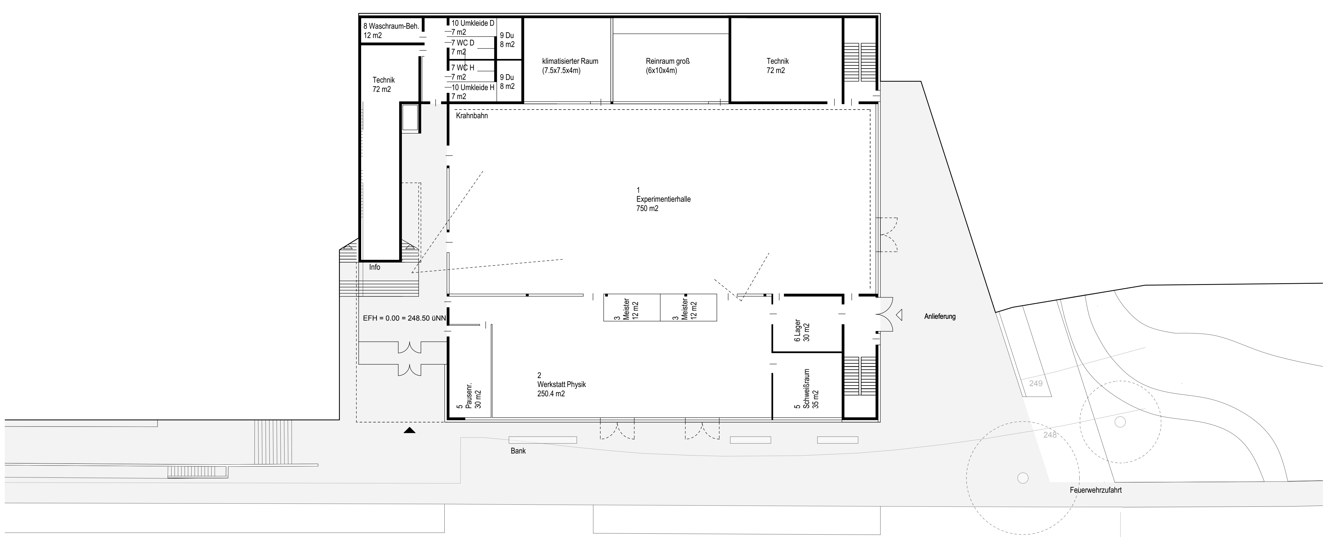
Grundriss E0 M 1_200
